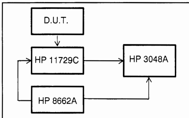
HP 3048A Phase Noise Measurement System extended to 18 GHz
