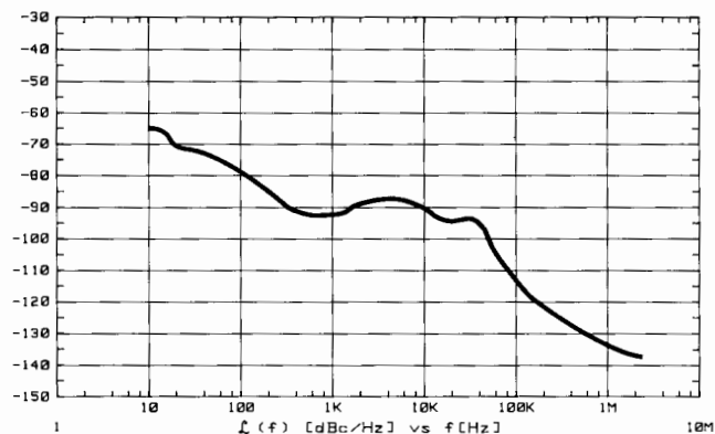
HP 8360 Phase Noise performance from 2.3 to 8.0 GHz
