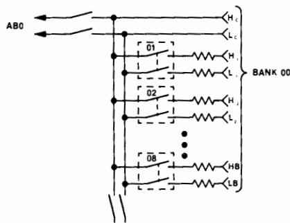
32 Channel Multiplexers (one bank shown)
