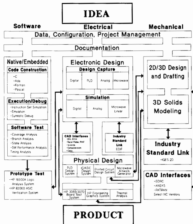
HP Open DesignCenter CASE/CAE/CAD Solutions
