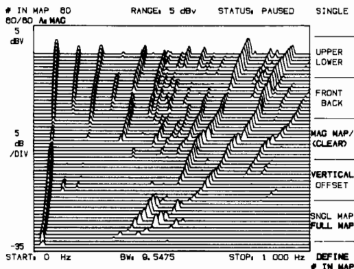
Spectral maps greatly reduce the time required to analyze changes in up to 60 successive measurements.
