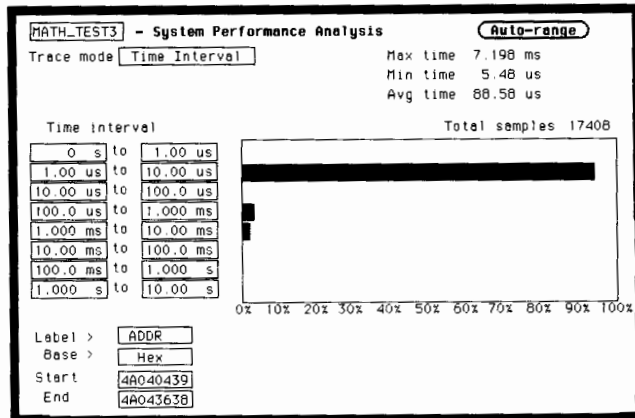
Time interval mode measures the time spent between two events in your system.
