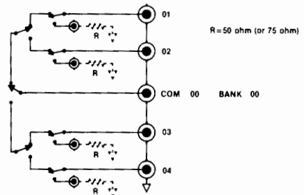
RF Multiplexer (one bank shown)
