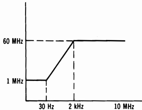
Figure 6 HP 5356D FM Tolerance
