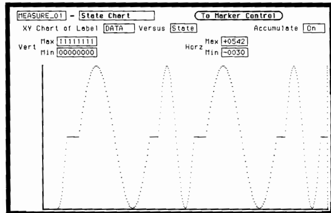
Plot label versus states to check A/D converters or memory coverage. Plot label versus label to obtain a circuit or routine "signature". Correlate chart display to inverse assembled listing.
