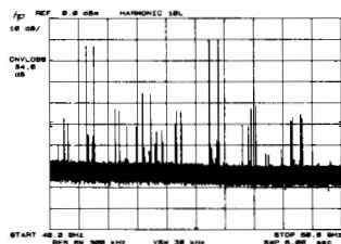
50-75 GHz sweep without preselection
