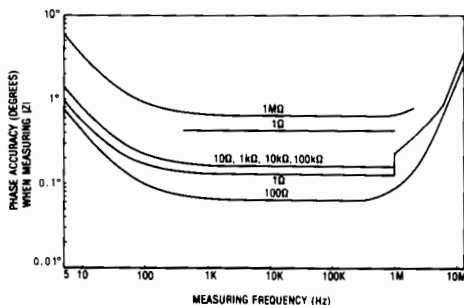
FIGURE 4: PHASE ACCURACY WHEN MEASURING |Z|
