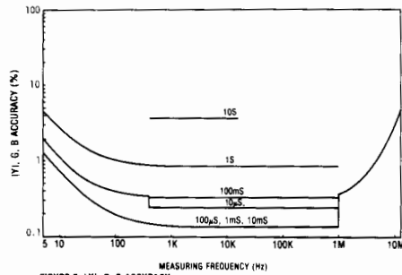
FIGURE 5: |Y|, G, B ACCURACY
