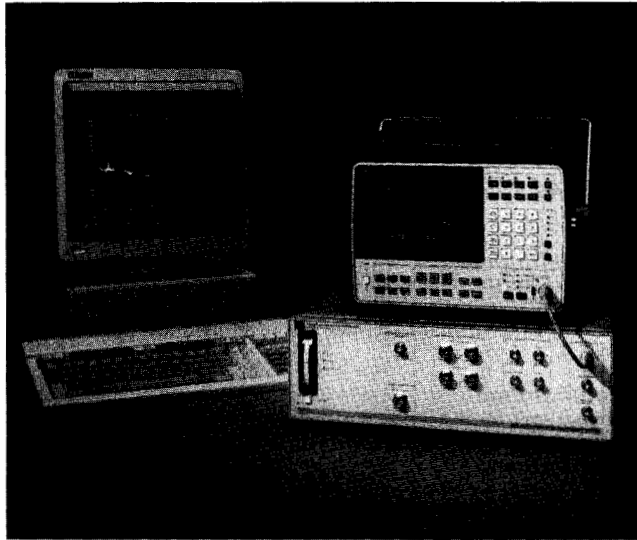
HP 3048A Phase Noise Measurement System controlled by an HP 98580C Desktop Computer.
