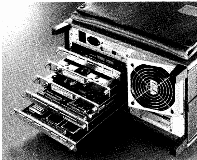
The HP 16500A supports 6 different measurement modules.
