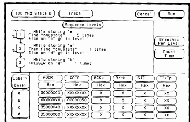
Trigger sequence capturing a write cycle on an 88000.
