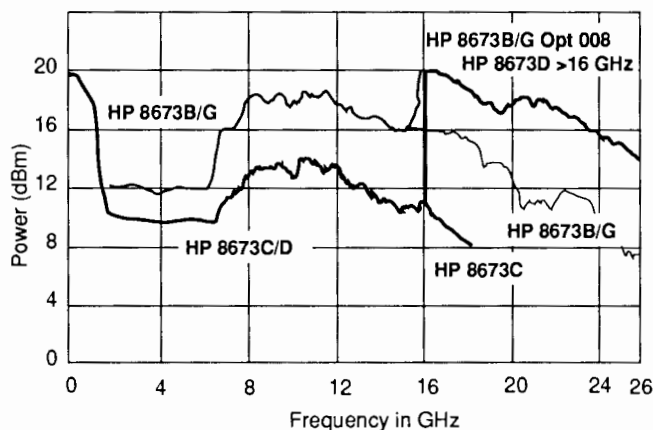
Figure 1. Maximum power typically available from HP 8673B/C/D/G and HP 8673B/G Option 008 at 25°C. HP 8673E and HP 8673H Option 212 and Option 618 typical maximum power is the same as HP 8673B/G over 2.0 to 18.0 GHz.
