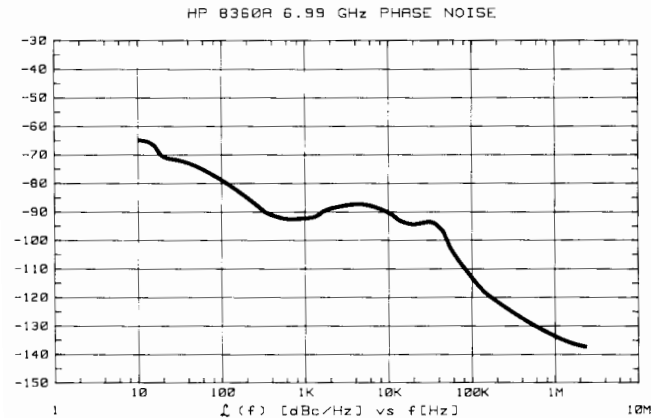
HP 8360A Phase Noise performance from 2.3 to 8.0 GHz
