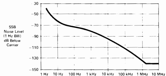
Typical HP 8673G single-sideband phase noise performance using the internal standard, Band 1.
