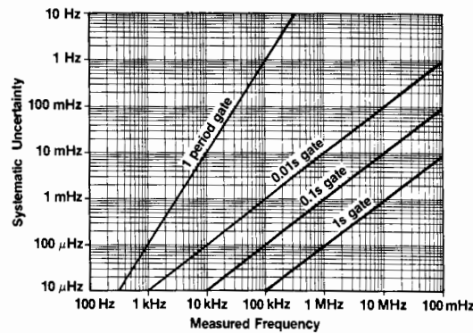
Graph 5. Internal uncertainties affect Frequency and Period measurements.
