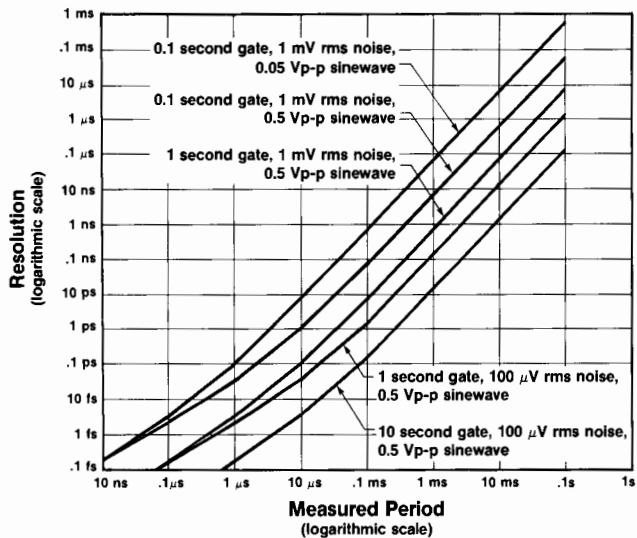
Graph 2. Period Resolution. Uncertainties which limit resolution can be reduced by increasing the gate time, reducing the noise on the input signal, or increasing the input signal amplitude.
