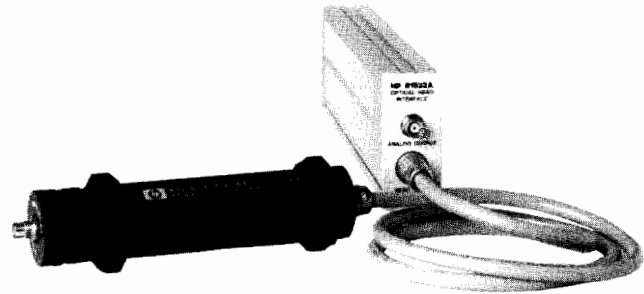
HP 81520A Optical Head with HP 8153A Optical Interface Module
