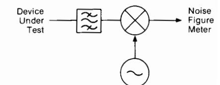
Single sideband noise measurement system.
