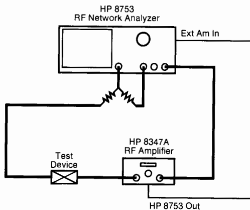
Extended Dynamic Range Configuration
