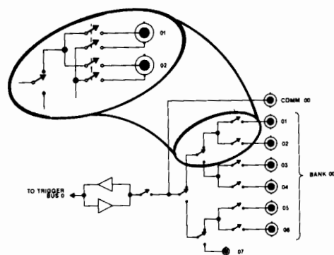
Switched-Shield Coaxial Multiplexer (one bank shown)
