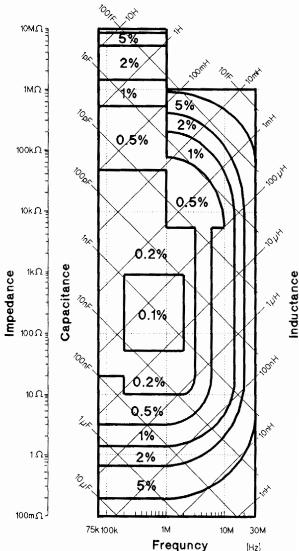
Figure 2. HP 4285A Measurement Accuracy
