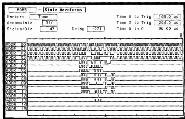
View an entire state acquisition at a glance to examine bus activity or processor control, fully correlated with state listing, X-Y chart and compare modes.
