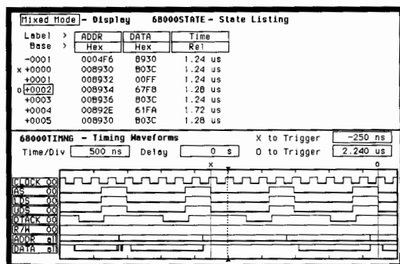
Time Correlated State and Timing Displayed on the Same Screen
