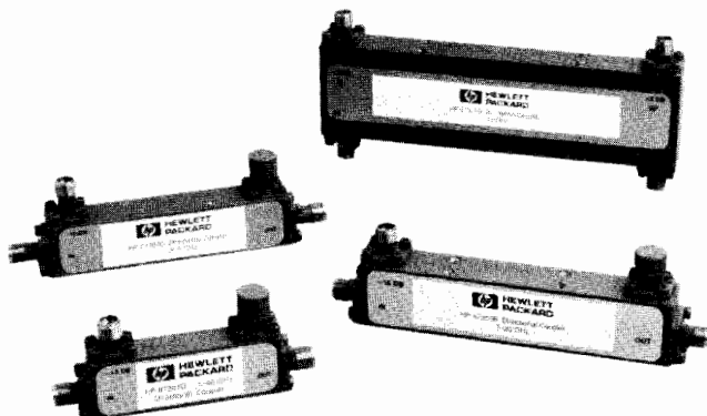
HP 87300B, 87301D, 87310B
